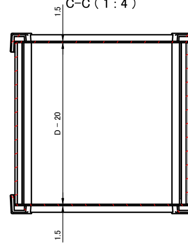
C-C (1:4)
