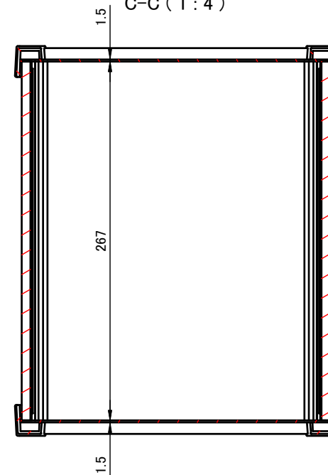
C-C (1:4)
