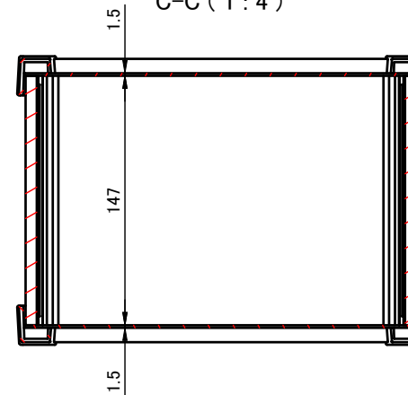
C-C (1:4)
