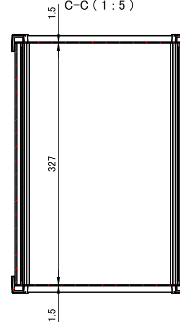
C-C (1:5)
