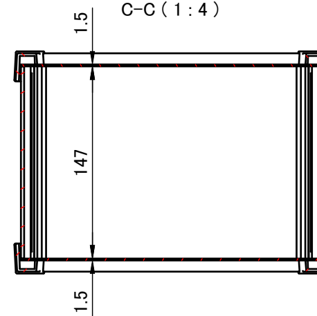
C-C (1:4)
