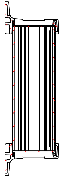
B-B (1:3)
