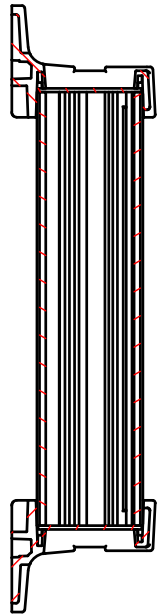
B-B (1:3)
