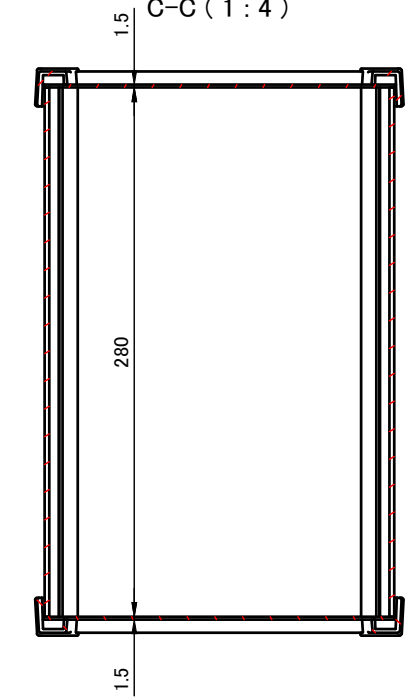
C-C (1:4)
