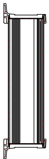
B-B (1:4)
