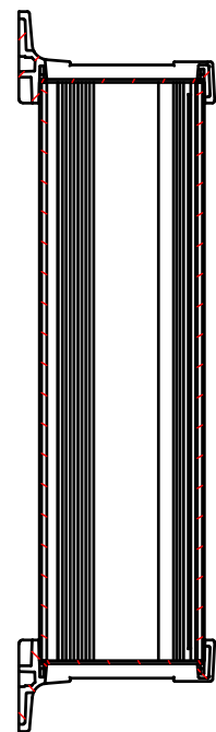
B-B (1:4)
