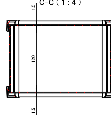
C-C (1:4)
