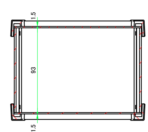
C-C (1:2.5)
