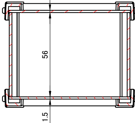
C-C (1:1.5)
