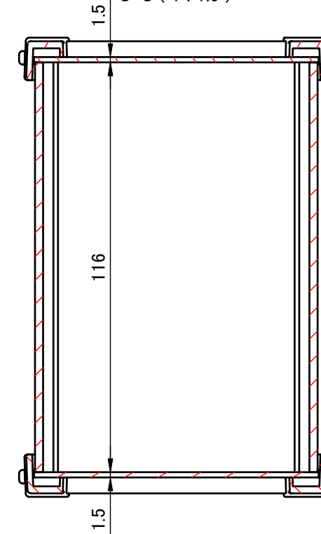
C-C (1:1.5)
