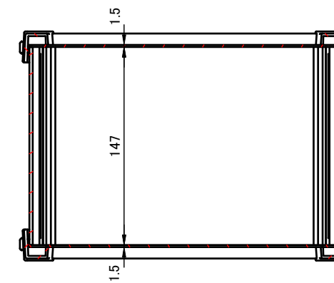
C-C (1:4)
