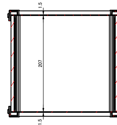
C-C (1:5)
