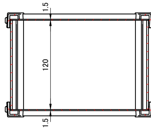
C-C (1:3)
