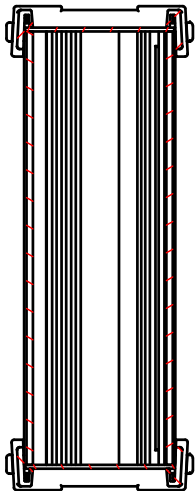
B-B (1:3)
