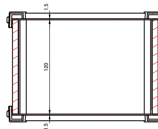
C-C (1:3)
