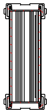
B-B (1:3)
