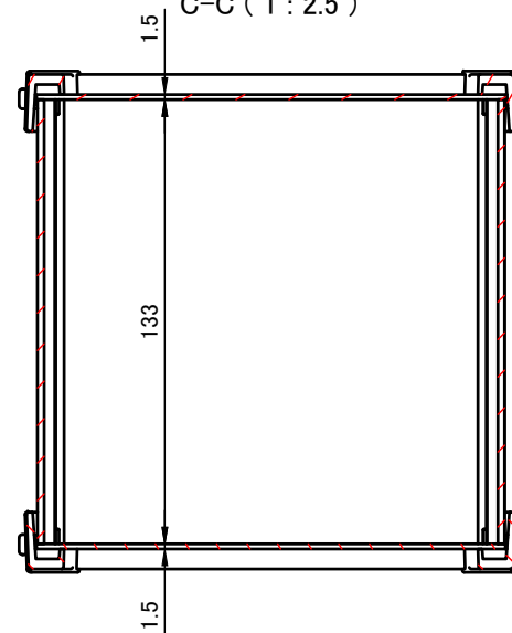
C-C (1:2.5)
