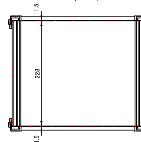
C-C (1:5)
