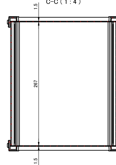
C-C (1:4)
