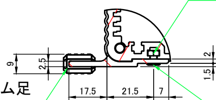
E (1:2) detail E
