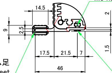
E (1:2) detail E
