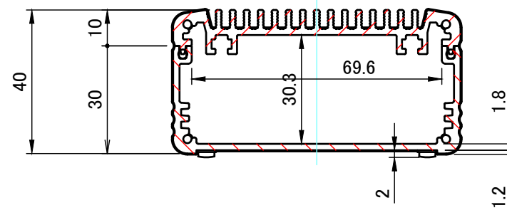
B-B (1:1.5)
