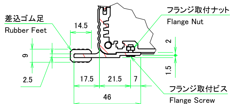
E (1:1.5) detail E
