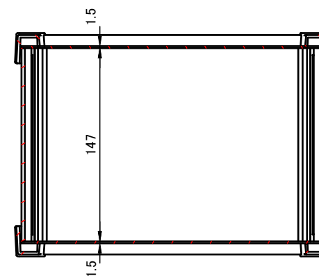
C-C (1:4)
