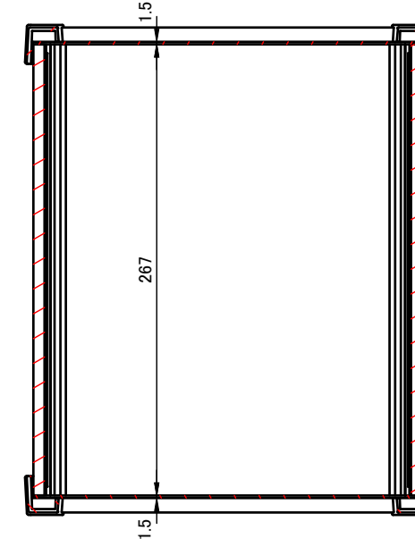
C-C (1:4)
