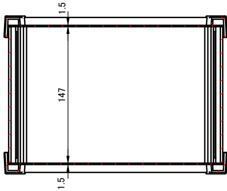
C-C (1:4)
