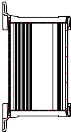
B-B (1:4)
