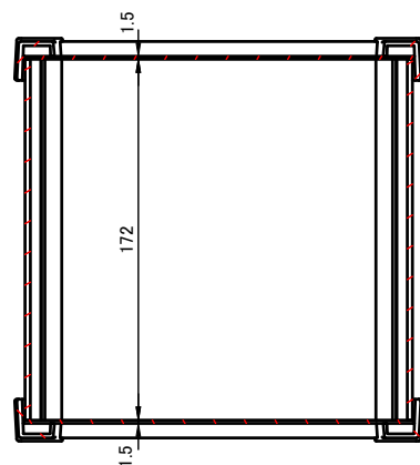
C-C (1:4)
