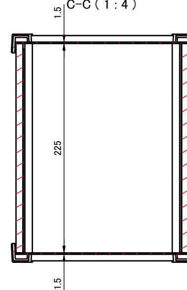
C-C (1:4)
