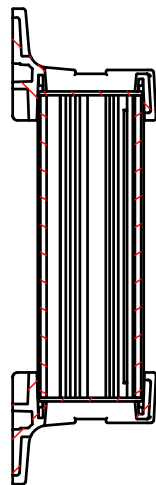
B-B (1:3)
