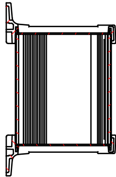
B-B (1:4)
