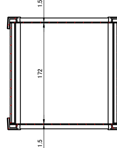
C-C (1:4)
