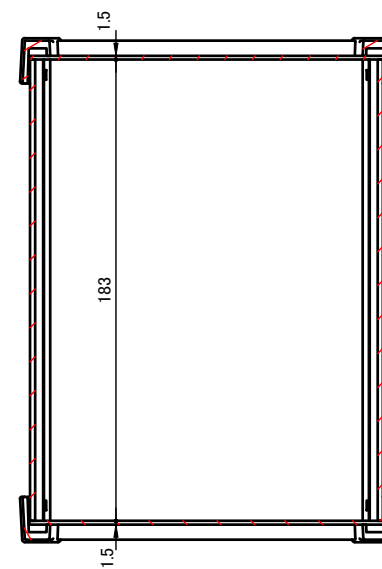
C-C (1:3)
