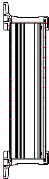
B-B (1:3)
