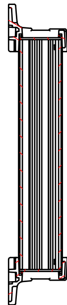
B-B (1:3)
