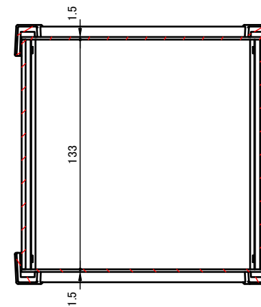
C-C (1:3)
