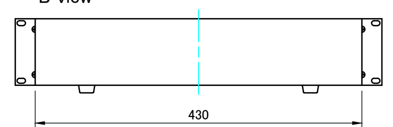
B view
