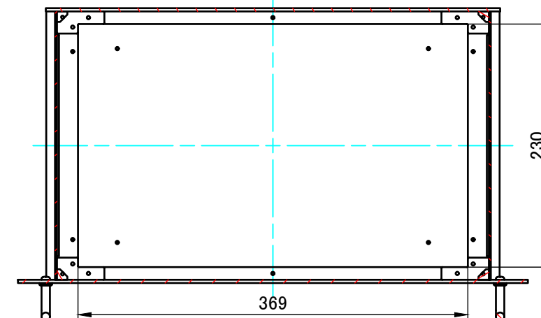
B-B (1:5)
