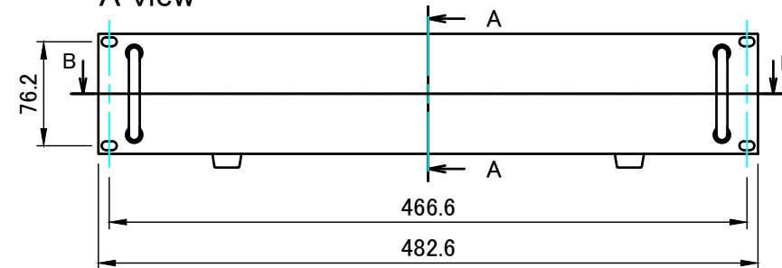
A view
