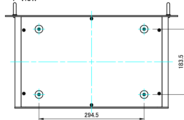
F view
