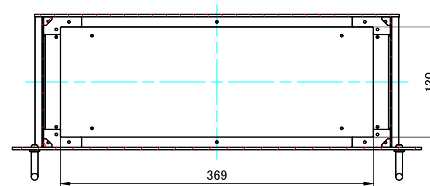
B-B (1:4.5)
