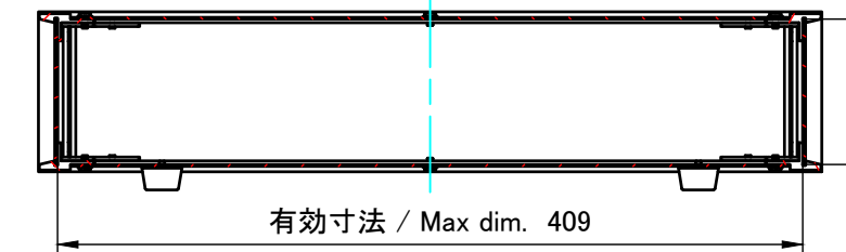
C-C (1:4.5)
