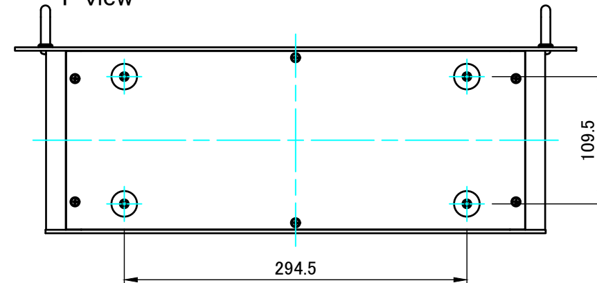
F view
