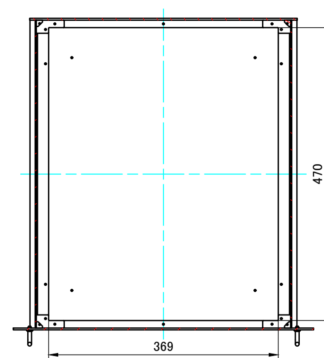
B-B (1:6)
