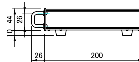
C view
