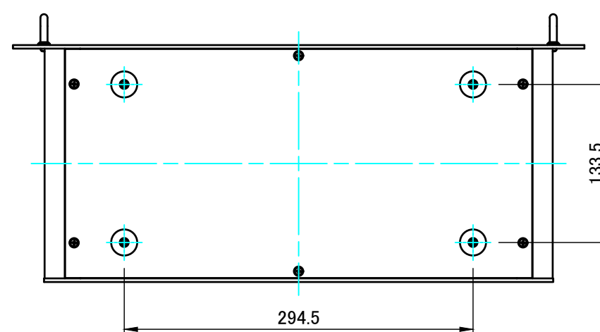
F view
