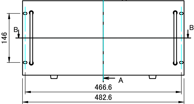
F view
