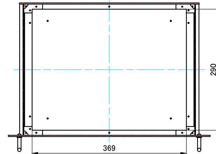
B-B (1:5.5)
