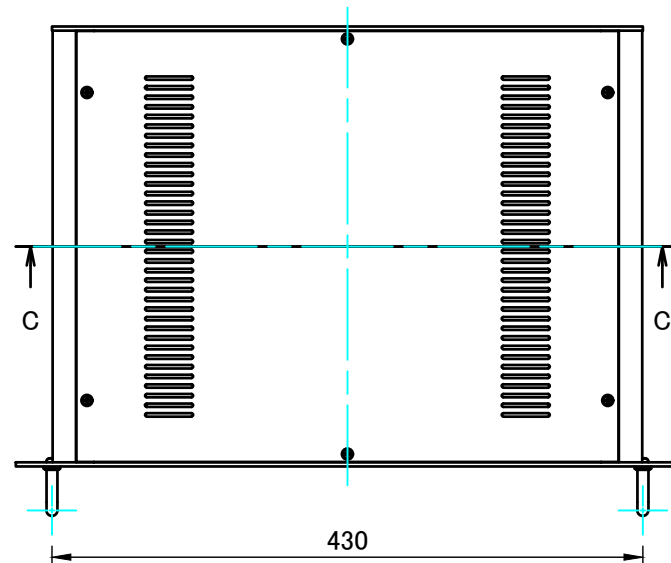
E view
