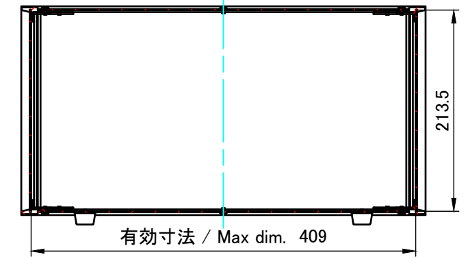
C-C (1:5.5)
