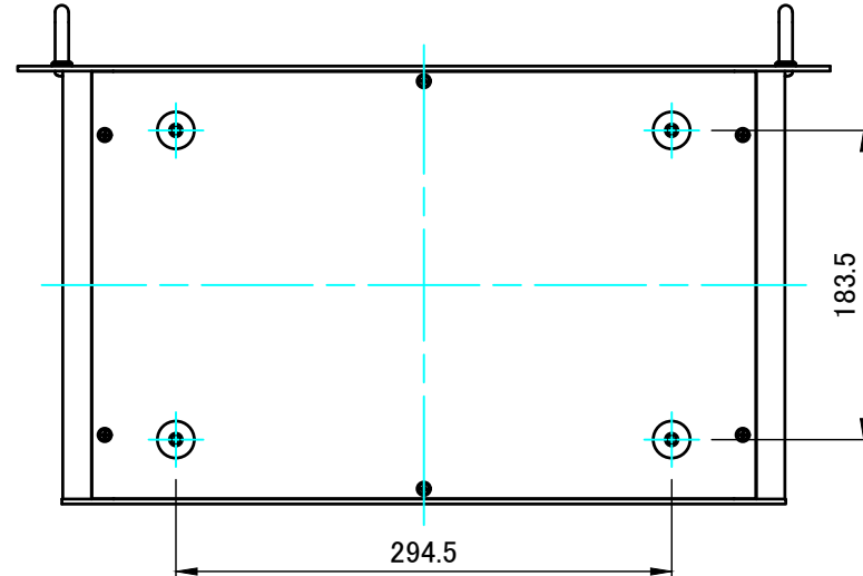
F view
