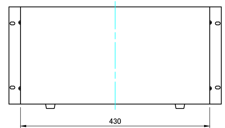
B view
