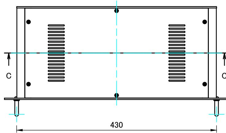
E view
