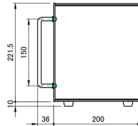
C view
