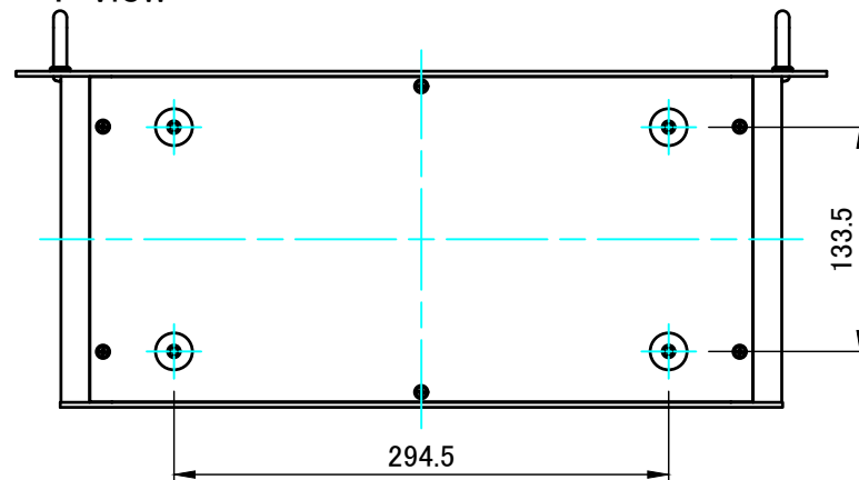
F view
