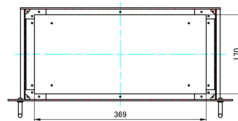
B-B (1:5)
