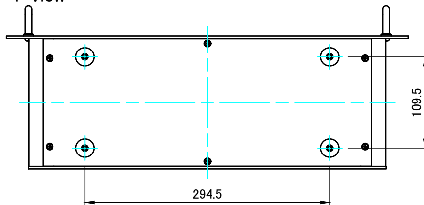
F view
