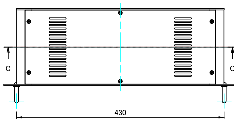
E view
