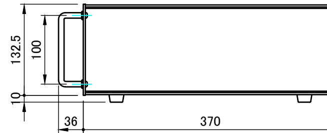
C view
