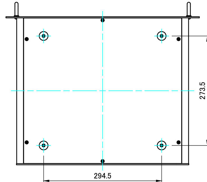
F view
