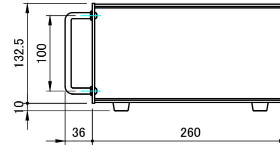
C view
