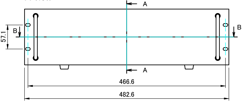
A view
