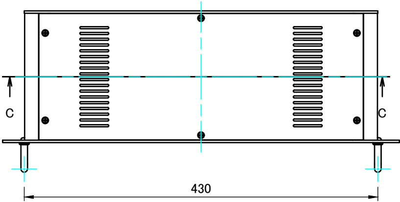
E view
