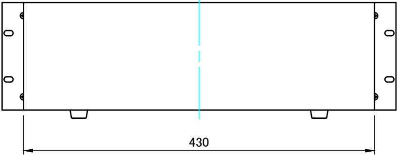
B view
