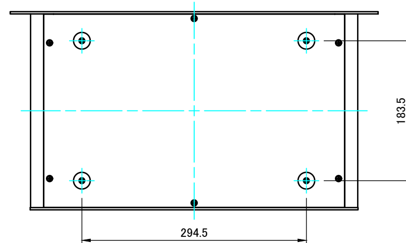
F view
