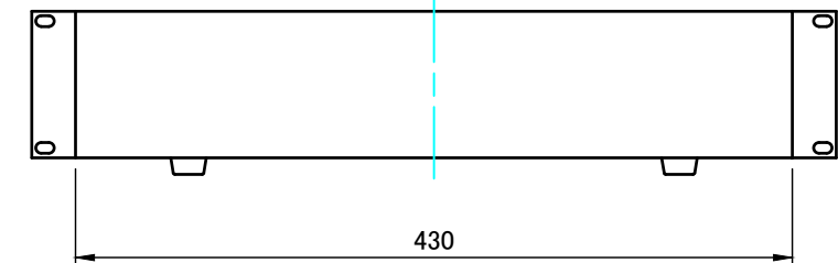
B view
