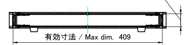
C-C (1:6)
